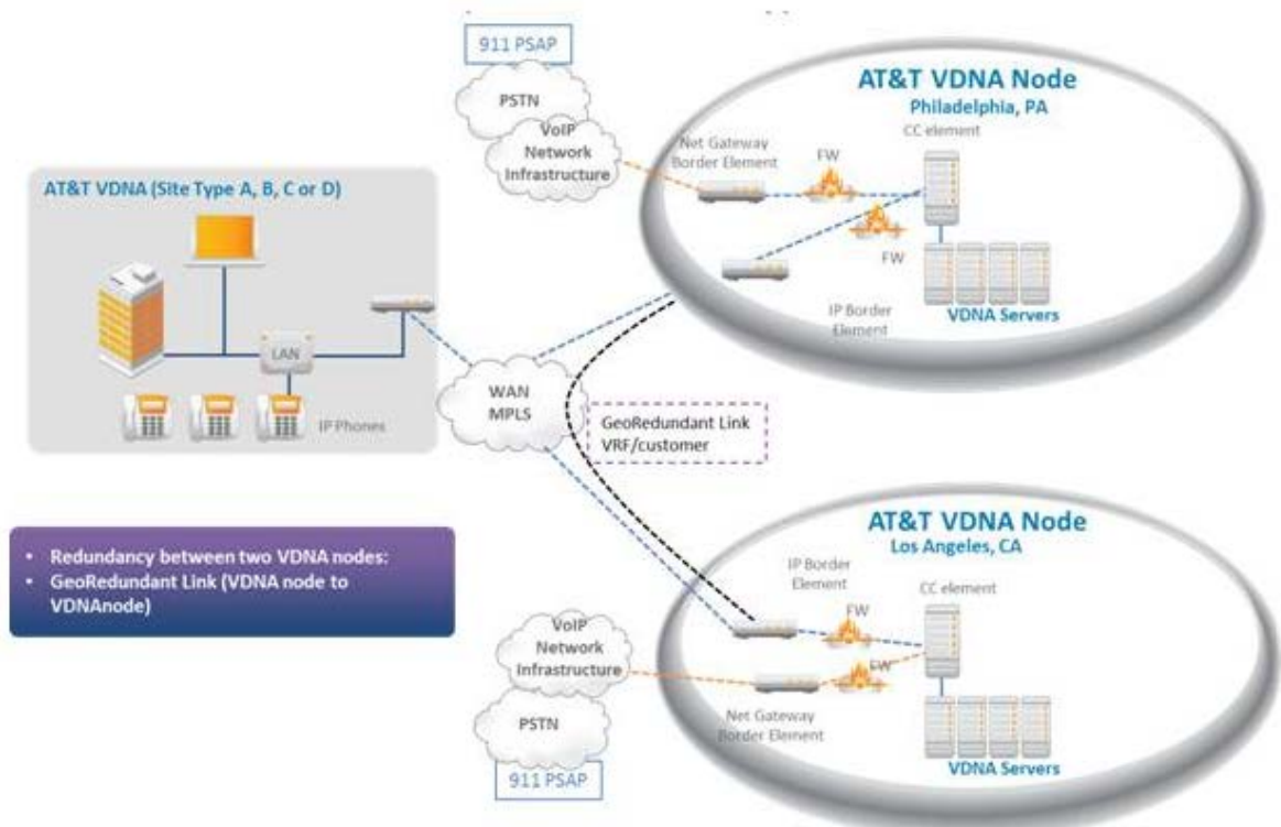
Figure 1.3-2. AT&T Voice DNA (Geo-Redundancy). Our Voice DNA hosted architecture is built with geo-redundancy.
